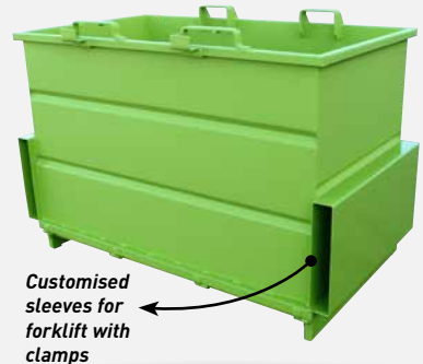
Lower lifting through fork sleeves
